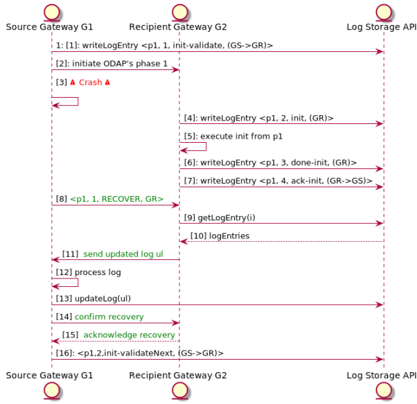
Fig. 3: \mathcal{G}_S crashing after issuing the init command to \mathcal{G}_R
