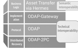
Fig. 1: The architecture of Hermes
